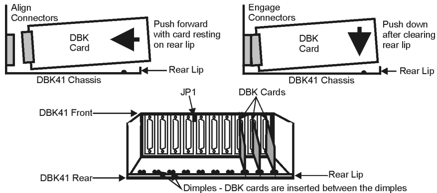
Inserting Cards into a DBK41
